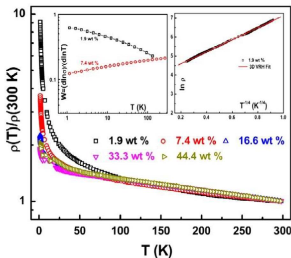
Fig. 8. Temperature dependence of normalized resistivity MWCNT–PVC composites MWCNT loading from 1.9 to 44.4 wt.%. Left inset. Reduced activation energy ( W ) vs. temperature ( T ) plot for 1.9 and 7.4 wt.% composites. Right inset. \ln(\rho) vs. T^{-1/4} plot for the 1.9 wt.% composite indicating the Mott-VRH mechanism of conduction. From ref. [21].
