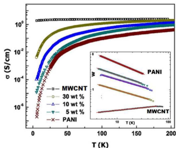
Fig. 6. Temperature dependence of conductivity of MWCNT and MWCNT–PANI composites. Inset. Reduced activation energy ( W ) vs. temperature ( T ) plots for MWCNT and composite samples. From ref. [43].
